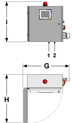
Control box
