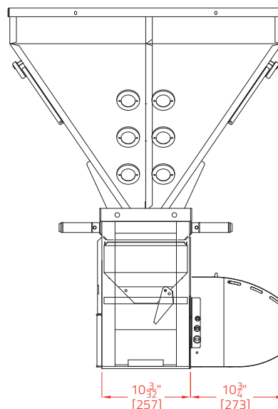
WXB-140 SIDE VIEW
