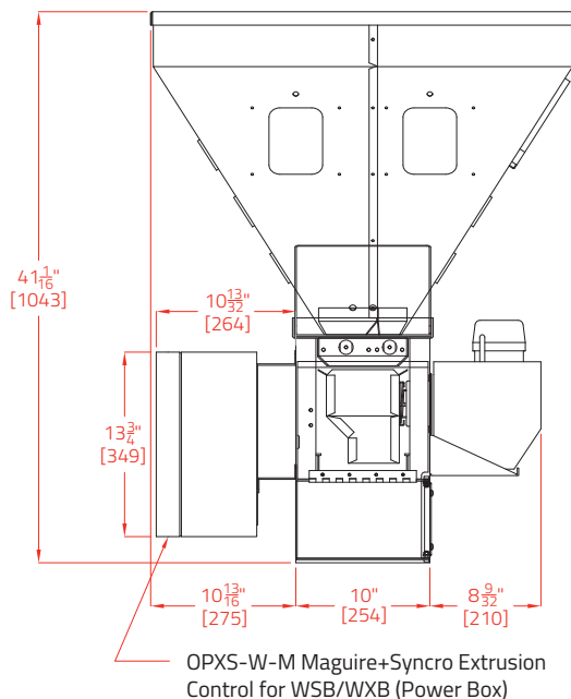
WXB-140 FRONT VIEW
